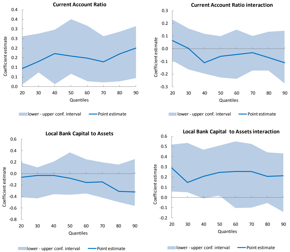
Figure 6b. Quantile Regression Setup: Macro Fundamentals and Bank Characteristics
