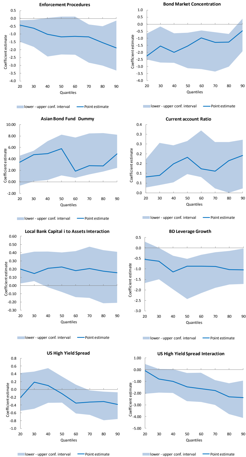
Figure 7. Quantile Regression Setup: Dropping Insignificant Regressors
