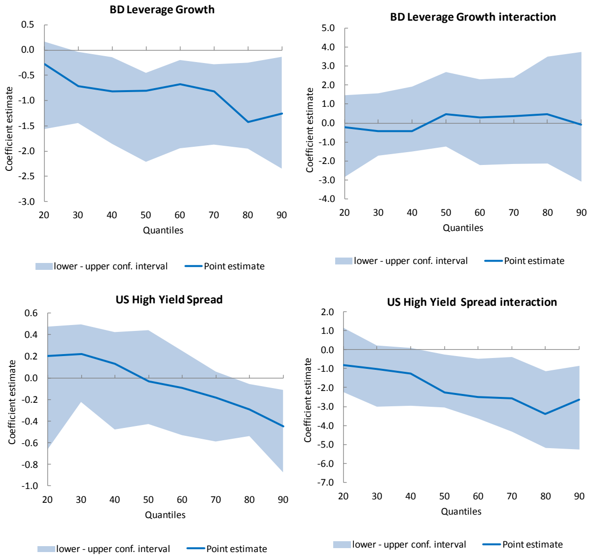
Figure 6c. Quantile Regression Setup: Global Factors
